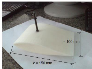
Figure 4. Airfoil equipped with wind tunnel attachment pin (chord and width measurements).
