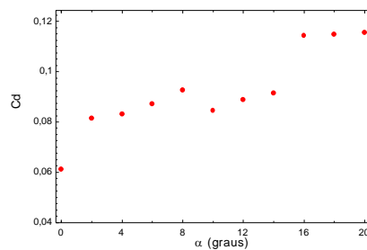
Figure 8. Drag coefficient versus angle of attack, Re=121200 .
