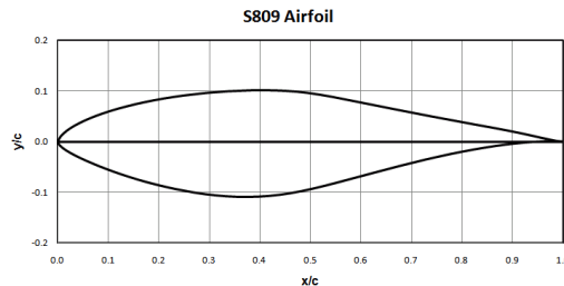
Figure 1. The profile of an S809 airfoil.
